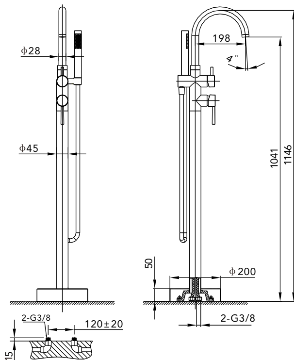
Installation drawing
