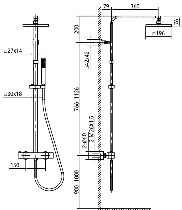
Installation drawing
