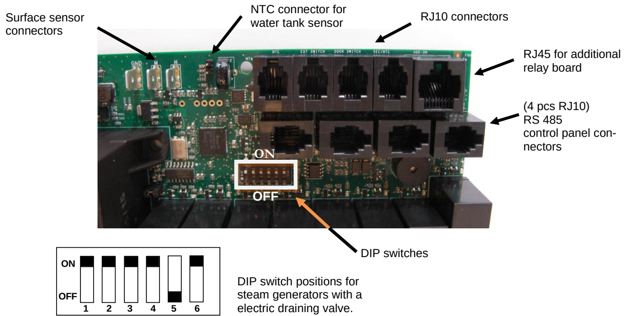
Switch diagram
