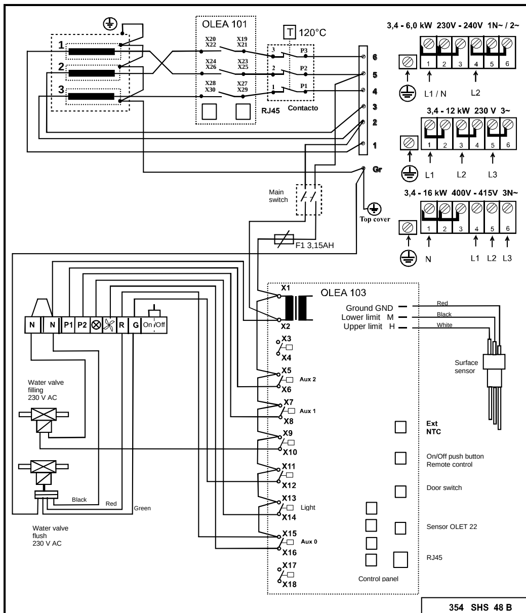
Switch diagram
