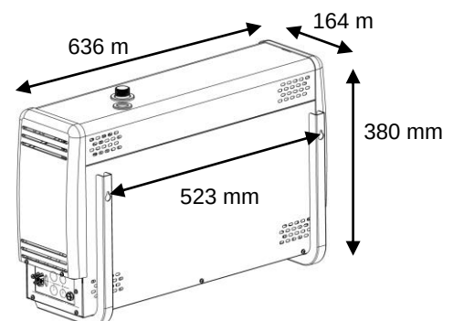
Wandmontage stoomgenerator
