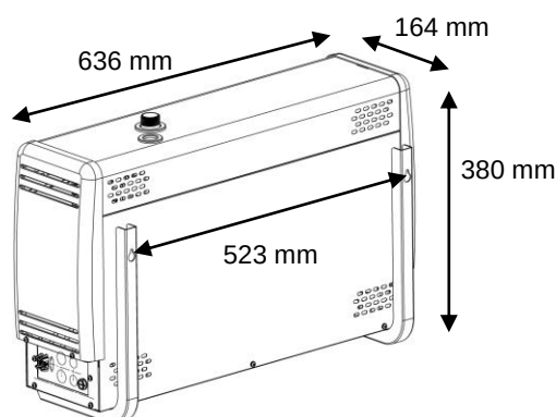
Steam generator wall mounting
