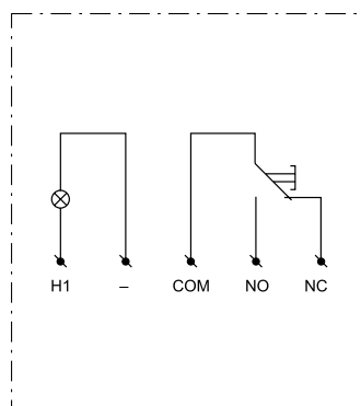
Pienjännitepainike PS1
