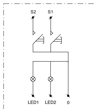
2-painike
