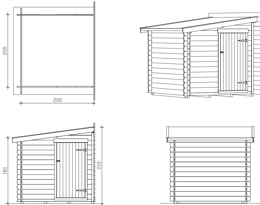
Floor plan, cross-section and elevations M 1:50
