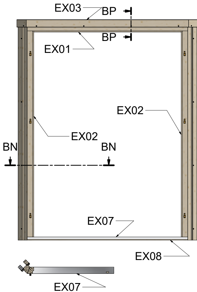
Specification Double Door Frame 40mm
